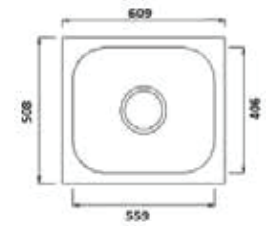
DRAINER WASTE
