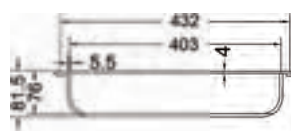
KA660002-CGL CONVEX RANGE TOWEL RAIL 18"
