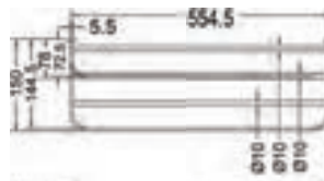
KA660010-CGL CONVEX RANGE TOWEL RACK 24"
