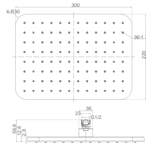
KA570034-CP RAIN SHOWER RECTANGLE (BRASS + ACRYLIC)
