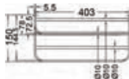
KA660011-CGL CONVEX RANGE TOWEL RACK 18"
