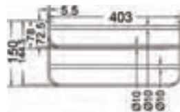
KA660011-CRG CONVEX RANGE TOWEL RACK 18"
