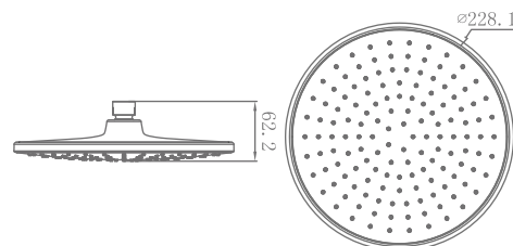
KA550022-MB SHOWER (ABS) + SHOWER ARM (SS)
