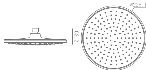
KA550022-CP SHOWER (ABS) + SHOWER ARM (SS)
